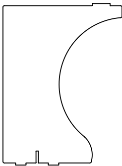
LARGE SUPPORT STAND (2 pcs)
